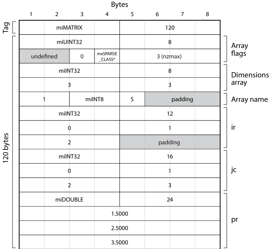
Figure 1-10, Example Sparse Array MAT-file Data Element
