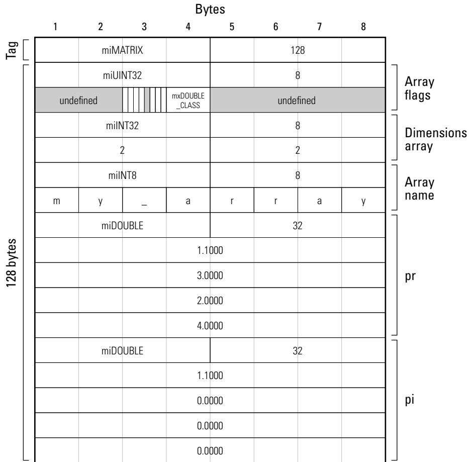
Figure 1-7, Example Numeric Array MAT-File Data Element Compressed Data Element
